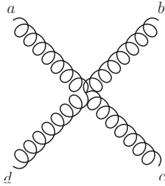
Figure 11: Three and four gluon vertices which arise from eq. (126). All momenta are taken to be incoming.
