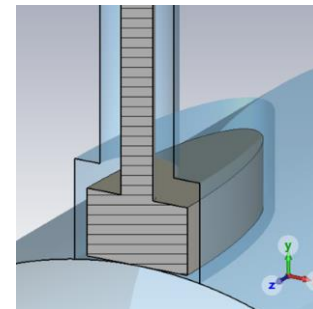
Fig 20: Elliptical button with ratio 4 modelled in CST, sliced at z=0.
