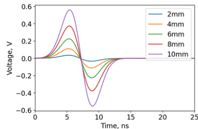
Fig 7: Voltage signal for different pickup radii, ttbar (SR) mode, with a 75 MHz filter applied.
