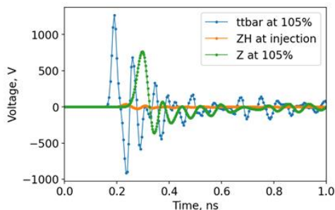
Fig 3: The voltage signal from a simplified pickup for the most extreme FCC-ee beams.
