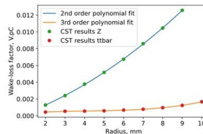
Fig 9: Wake-loss factor vs pickup radius.
