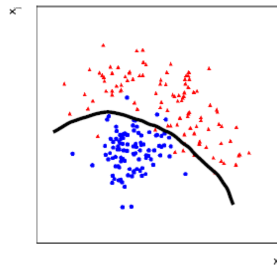
good trade-off
