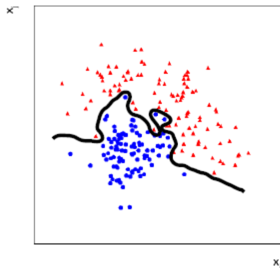
overtraining
